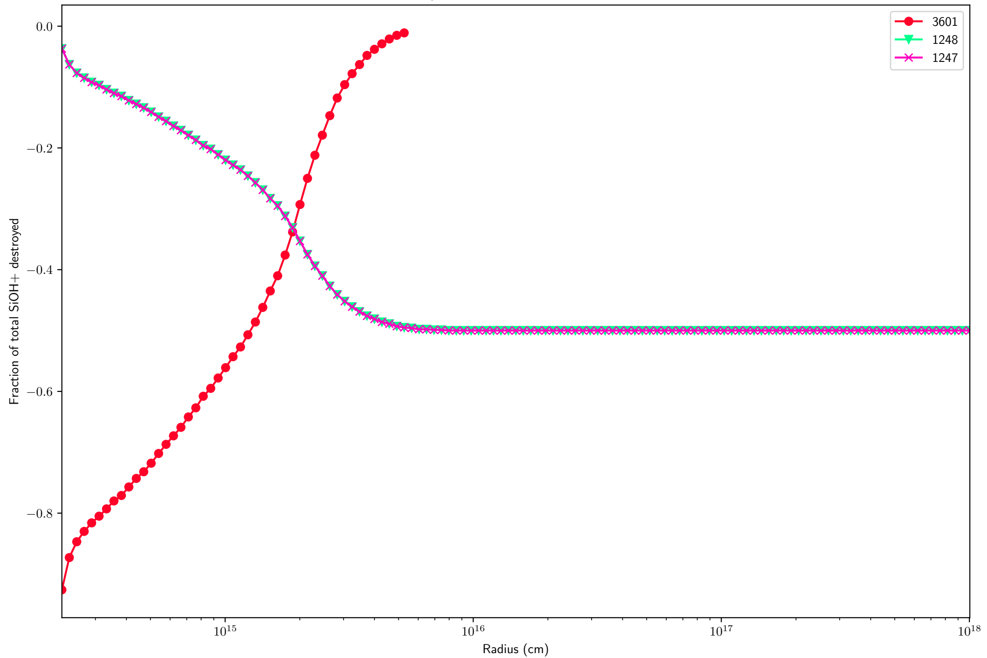
destruction-major-1-SiOH+-model-2025-10-28h12-30-45
